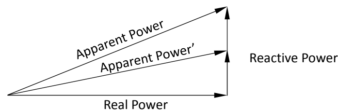
Figure 1: Power triangle for Apparent Power, Real Power and Reactive Power (Note: Apparent Power' refers to the apparent power after power factor correction)
