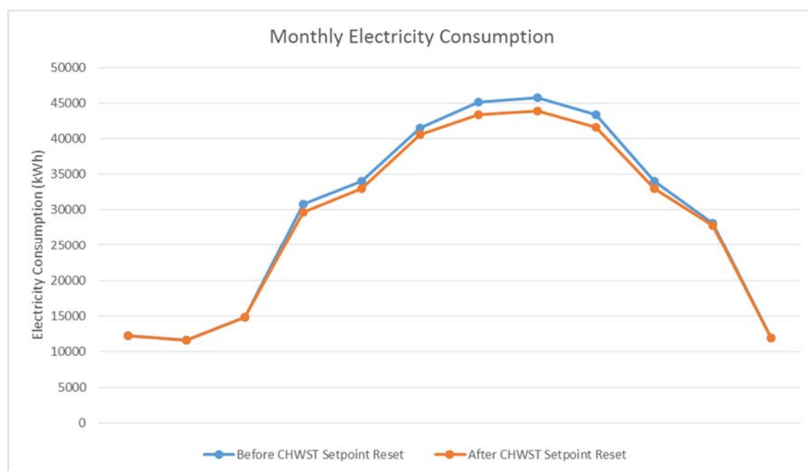
Figure 3d) Monthly Electiricty Consumption Before and After CHWST Setpoint Reset
